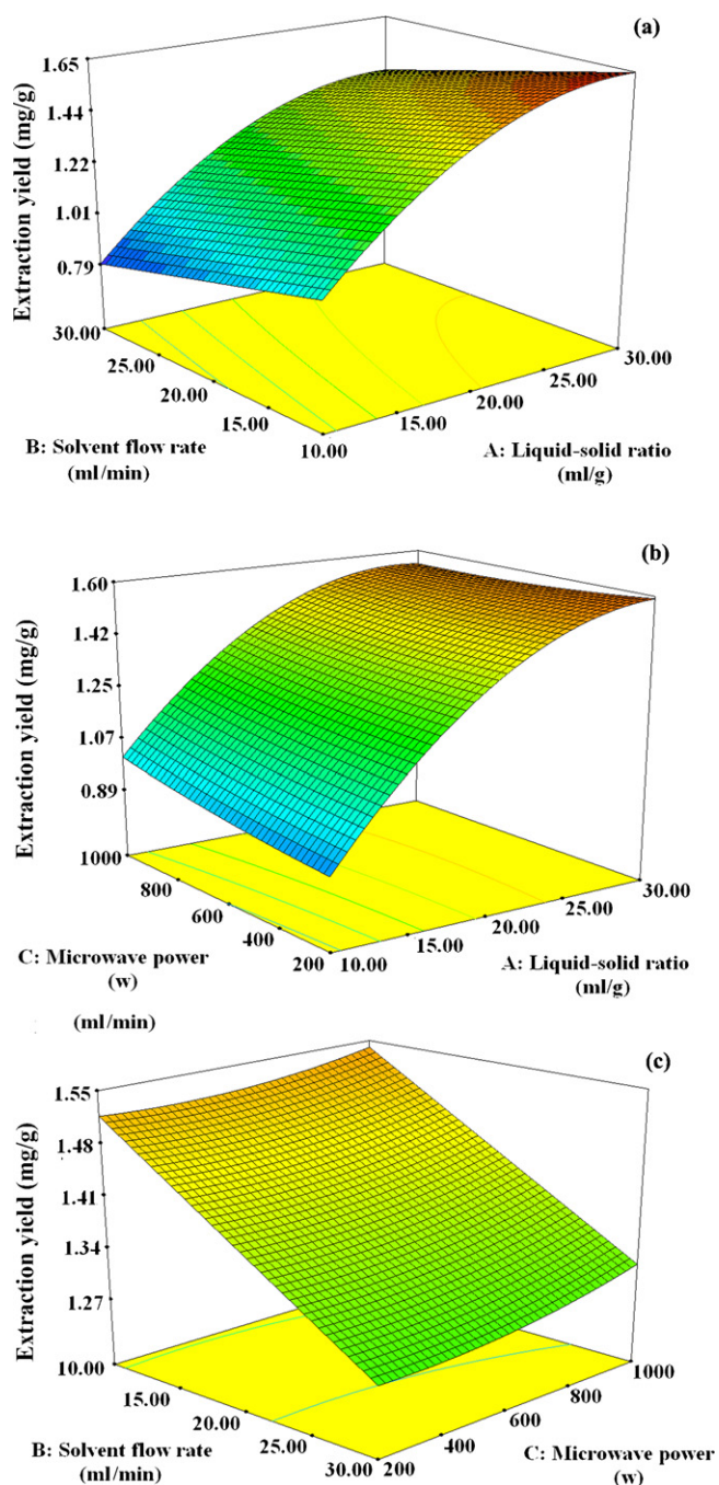
Fig. 4. 3D-surface plots showing the effects of: (a) liquid-solid ratio (ml/g) and solvent flow rate (ml/min); (b) liquid-solid ratio (ml/g) and microwave power (w); (c) solvent flow rate (ml/min) and microwave power (w).
