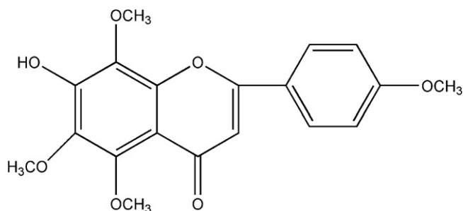
Fig. 1. The chemical structure of nevadensin.
